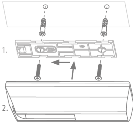
Mounting directly on the ceiling
